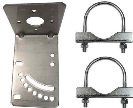
Includes Tilt L-Bracket Mount w/ 2 U-Bolt Sets
